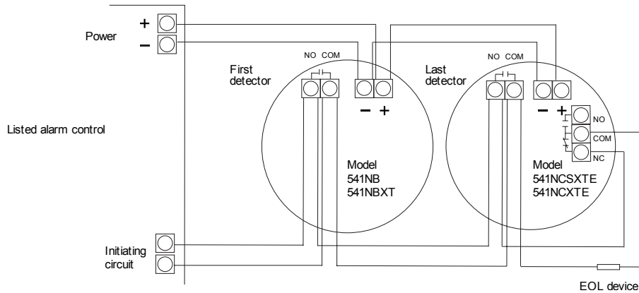
Figure 8: 500N series four-wire E model wiring
